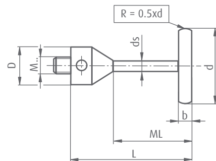
Disc probe
