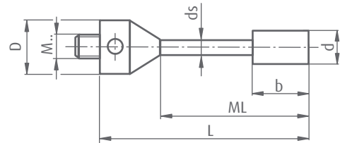
Cylinder probe
